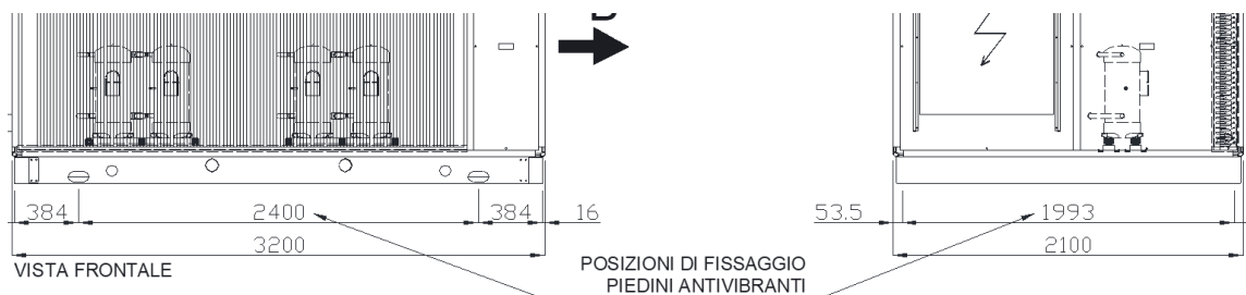
Rubber antivibration dampers
