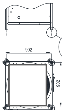
Antivibrante in gomma Rubber antivibration dampers
